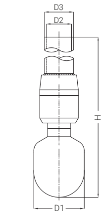
UBC welded connection
