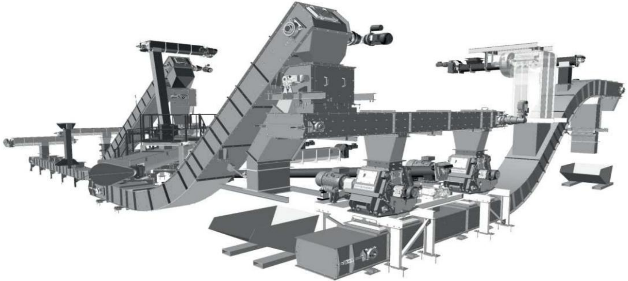
Transport of ash and slag from under the boiler
