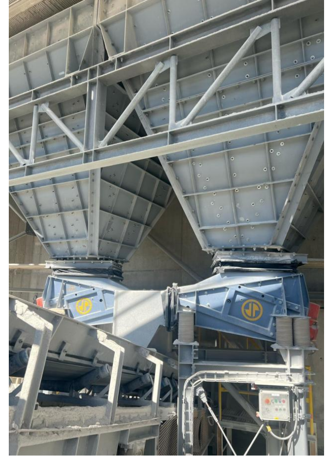
Wagon unloading station for limestone with downstream conveying
